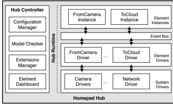
Figure 7. HomePad hub architecture.
